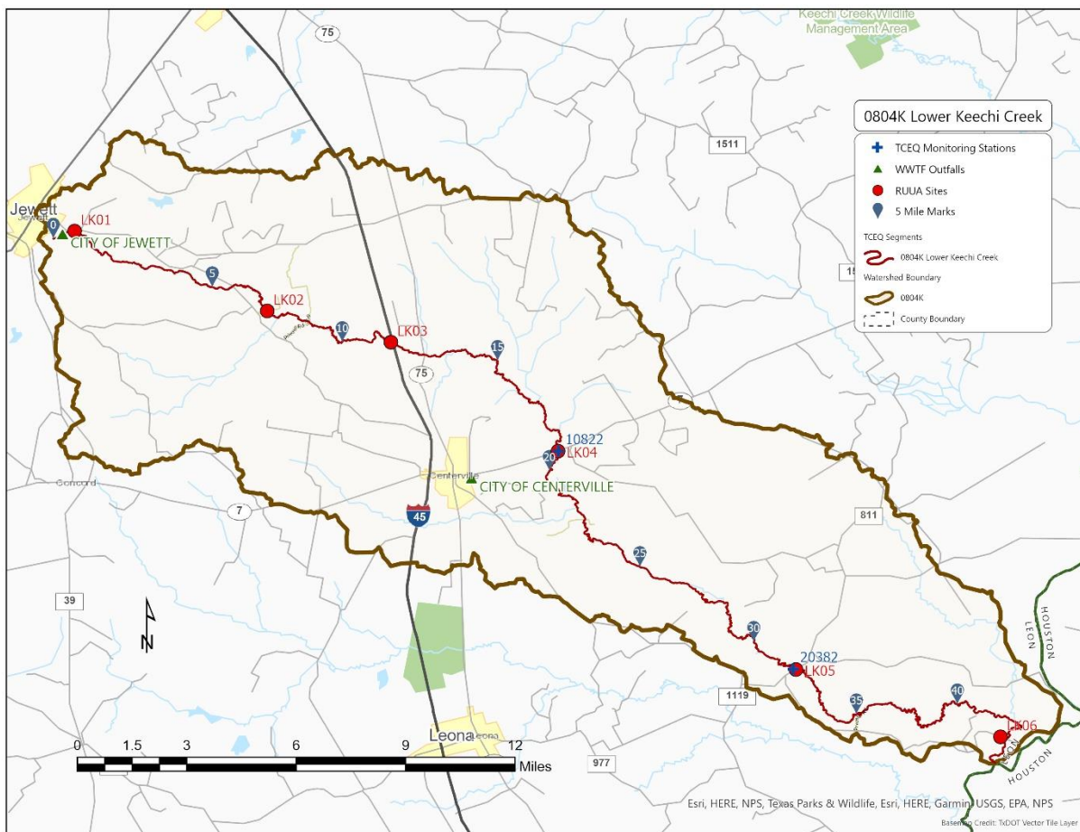
Figure 4.13 Summary of observed and interviewed human activities on Lower Keechi Creek
